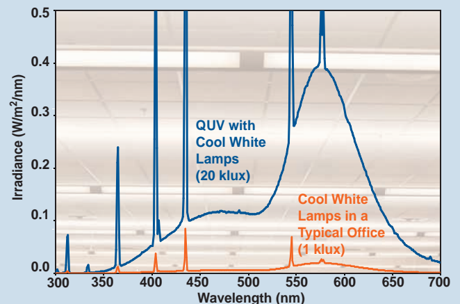
The QUV/cw uses cool white lamps to simulate indoor environments, such as the overhead fluorescent lighting typically found in offices. It also meets ISO, ANSI and ASTM test methods for indoor photostability testing.
